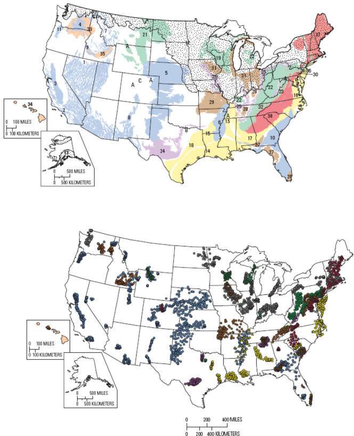
Figure 3 : (A) Principal aquifers of the United States and major aquifer groups used in the current study, and (B) wells sampled by the National Water-Quality Assessment Program, 1992–2003, color coded by aquifer (see explanation). Areal extent of aquifers from U.S. Geological Survey (2003).
